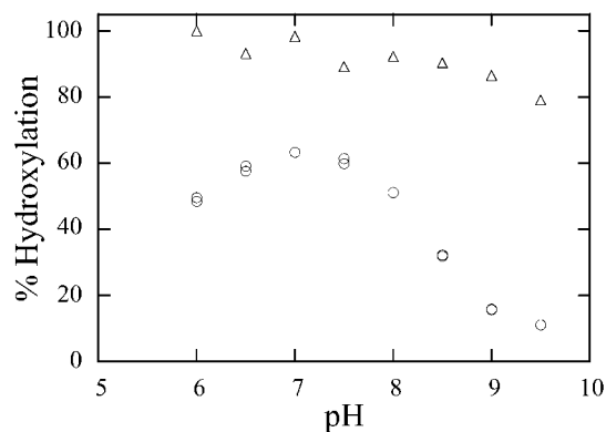
FIGURE 5: Variation of hydroxylation efficiency with pH. Hydroxylation efficiency, defined as 100 \times (\text{pOHb hydroxylated}) / (\text{NADPH consumed}) , was determined by measuring the amount of NADPH consumed in steady-state assays at 25 °C in the presence of limiting amounts of pOHb. Protocatechuate dioxygenase was included to prevent PCA-stimulated NADPH consumption by PHBH. Values obtained for the wild-type enzyme are shown by triangles, while values obtained for the Pro293Ser mutant are shown by circles.
