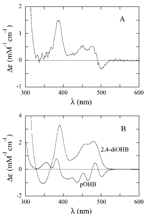
FIGURE 3: Difference spectra caused by the binding of benzoate ligands. Panel A shows the spectral perturbations caused by the binding of pOHB to the Pro293Ser mutant (9.1 \mu\text{M} ) in 50 mM KPi, 0.5 mM EDTA, pH 6.5, at 4 ^{\circ}\text{C} . Panel B shows the difference spectra for the wild-type enzyme caused by the binding of pOHB and 2,4-diOHB.
