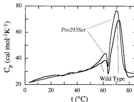
FIGURE 2: Thermal denaturation of PHBH. DSC traces of the irreversible melting of the wild type and Pro293Ser enzymes are shown. The enzyme concentration (900 \mu\text{M} ) was the same in both experiments. DSC experiments were conducted in 50 mM KPi, 0.5 mM EDTA, pH 6.5, using a scan rate of 1 °C/min.
